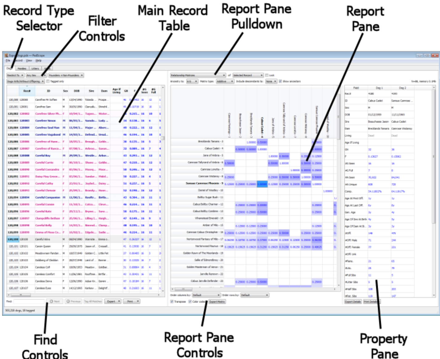
PedScope Main Window
